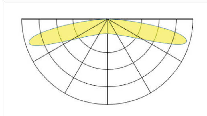
Beam angle: 175°
